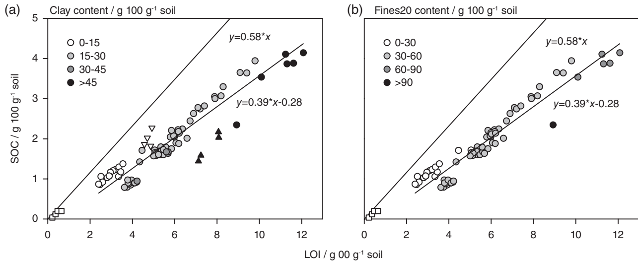
Figure 1 Soil organic carbon (SOC) as a function of loss-on-ignition (LOI) for (a) samples grouped by soil clay content ( n = 88 ) and (b) samples grouped by soil mineral particles < 20 µm (Fines20) content ( n = 80 ). The clay- (< 2 µm), silt- (2–63 µm) and sand-sized (63–2000 µm) fractions from the Lerbjerg site are shown with triangle up, triangle down and square symbols, respectively. Because of different size limits for silt isolated from Lerbjerg, panel (b) does not include Fines20 from Lerbjerg. The line representing the conventional relation between LOI and SOC ( SOC = 0.58 \times LOI ) is also shown.
