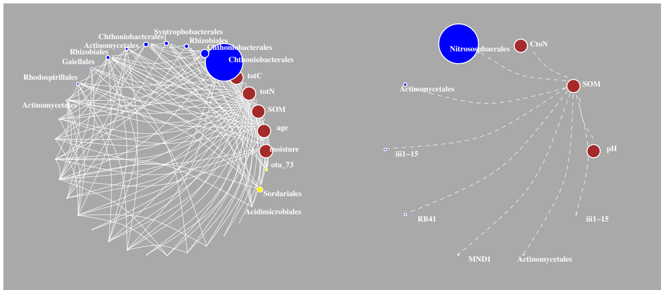
FIGURE 6 Network analysis of full dataset (soil chemistry, functional and biodiversity indicators) showing only strong correlations with SOM content. The left panel shows variables positively correlated with SOM ( > 0.7 ) and the right panel shows negative correlations ( < -0.7 ). For the molecular indicators the size of nodes is scaled to relative OTU abundance, and only the more abundant taxa are labelled. Blue nodes represent bacterial taxa, red nodes represent soil properties and yellow nodes are fungal taxa
