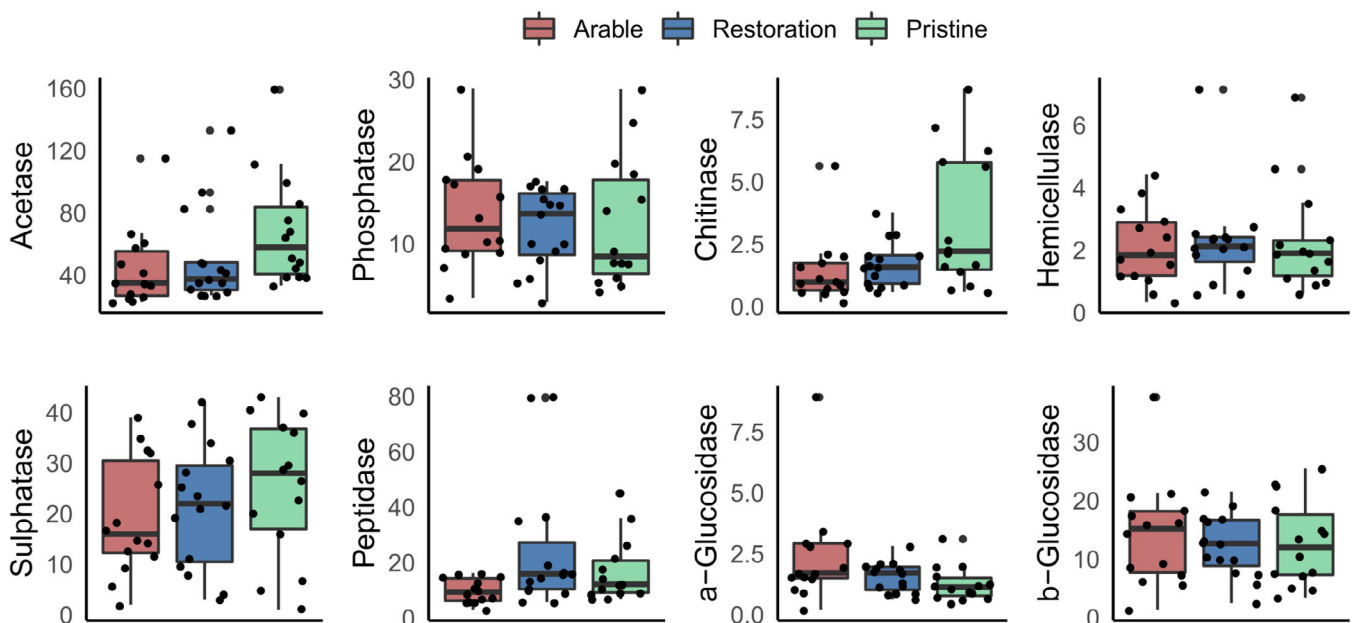
FIGURE 3 Eight hydrolytic soil extracellular enzymatic activities in nkat (nanomol substrate degraded per minute, normalized per gram dry soil) as response to land use in a calcareous grassland restoration chronosequence. Acetase, Chitinase, \alpha - and \beta -glucosidase and hemicellulase activities are considered to be relevant for carbon compound degradation, whereas phosphatase (aryl-phosphatase) is involved in P cycling and peptidase (leucine-aminopeptidase) catalyses degradation of nitrogen compounds (peptides)
