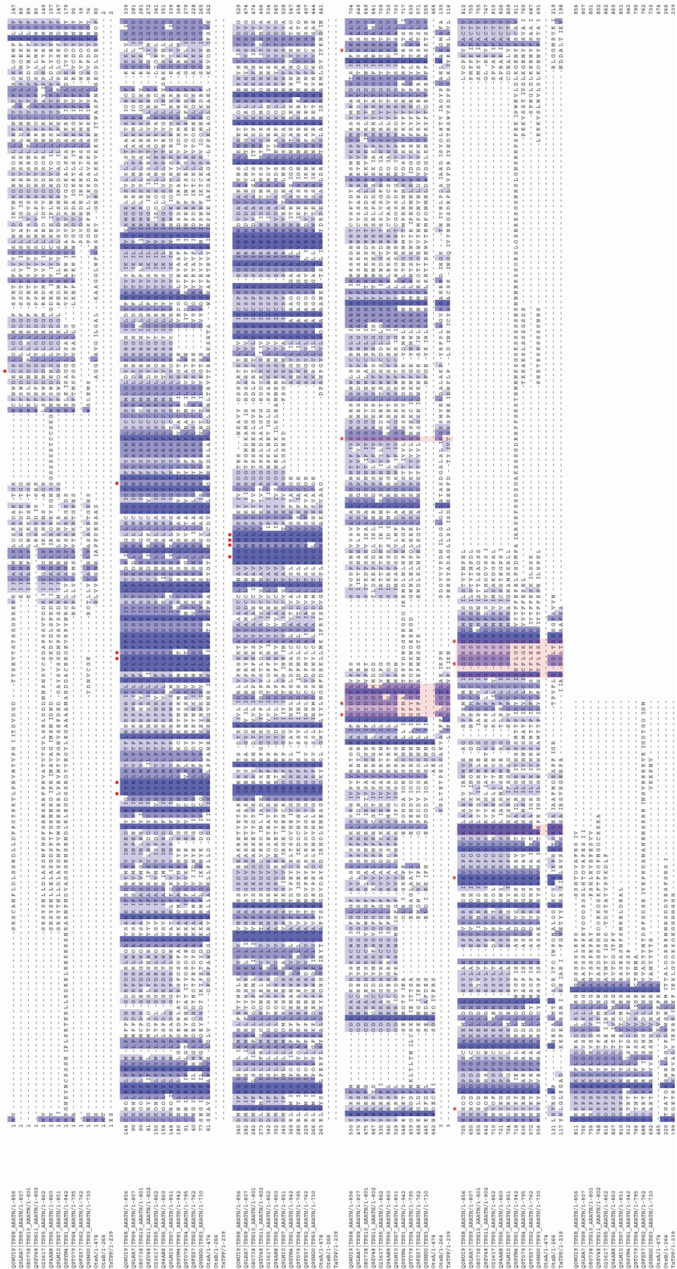
Figure 3. Alignment of Arabidopsis TPS proteins with E. coli OtsA (TPS), OtsB (TTP) and Thermoplasma acidophilum TPP (TaTPP).
