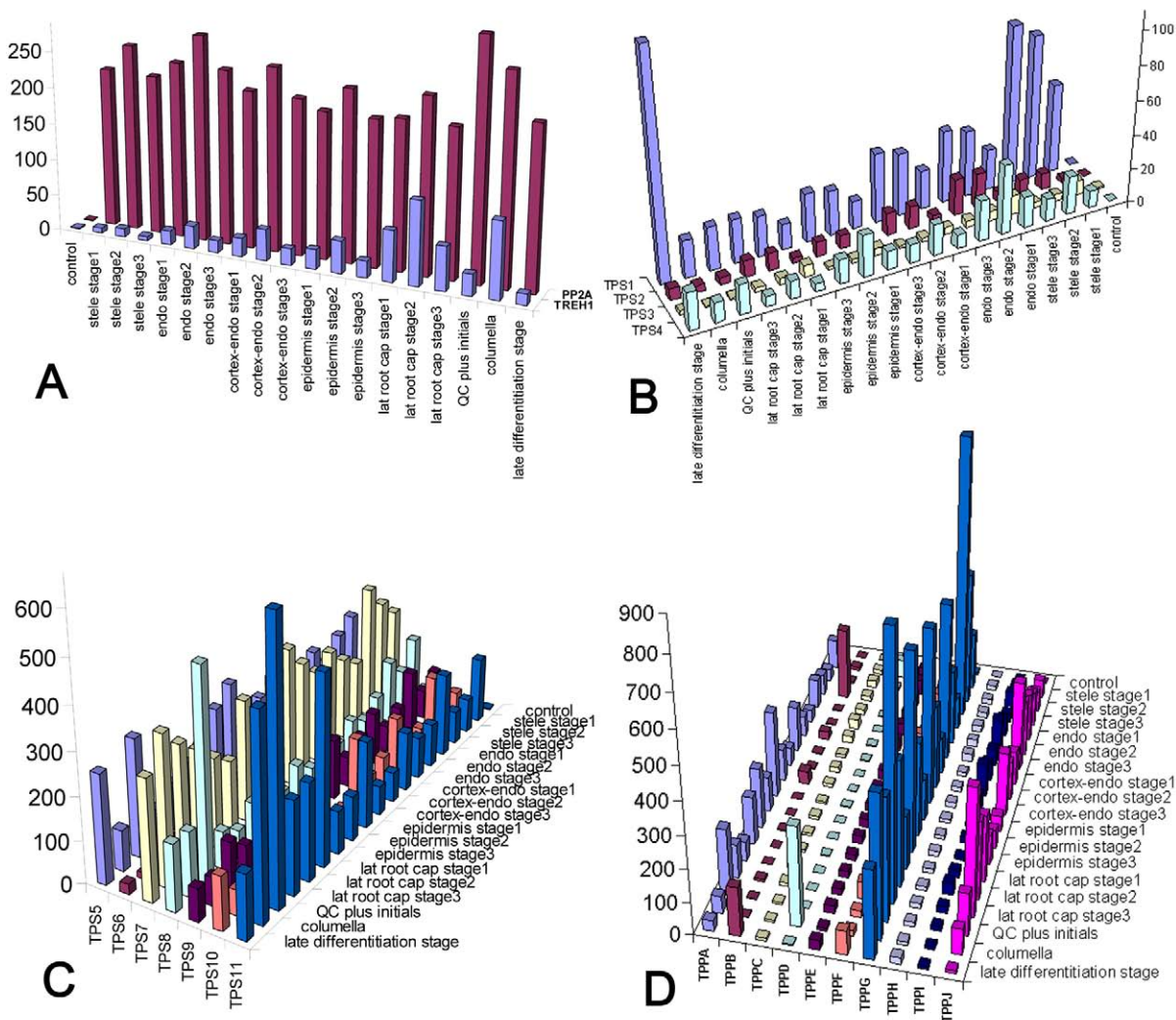
Figure 5. Expression of genes associated with trehalose metabolism in protoplasts of different root tissues. Data are from (Birbaum et al., 2003; Brady et al., 2007); tissue identities are defined in these references.
