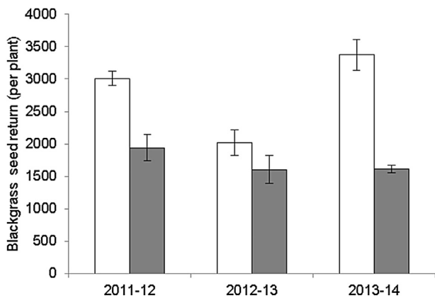
Fig. 4. The seed return per plant of A. myosuroides (approx. 80 plants m -2 equiv.) when grown alongside one of two cultivars (275 plants m -2 equiv.) across three years in a container-based experiment. ■ = Duxford; □ = KWS Santiago. Mean temperature in 2011–12 was 8.3 °C, in 2012–13 was 6.3 °C and in 2013–14 was 8.9 °C.
