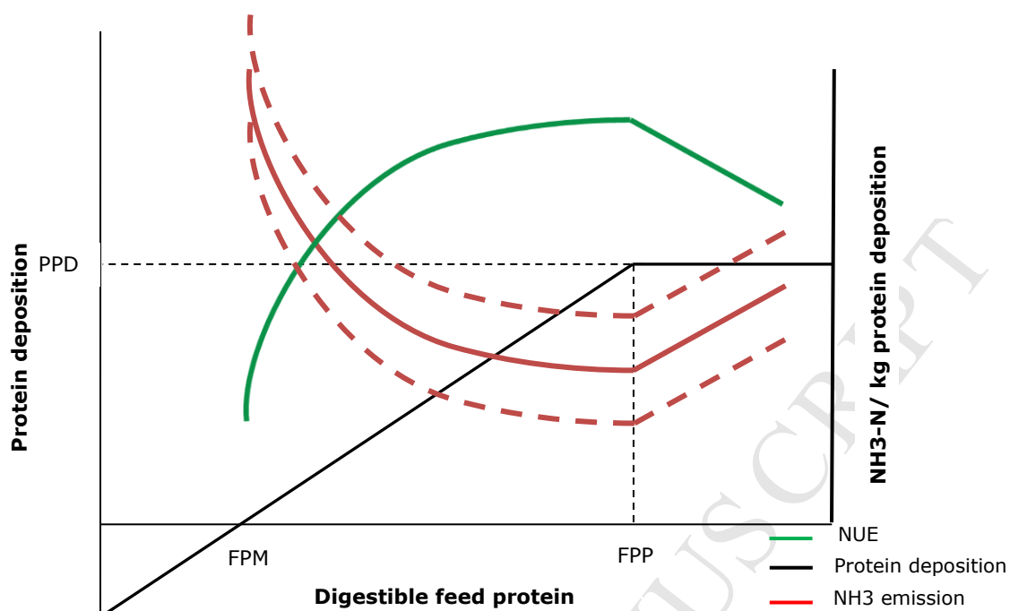
Figure 2. Protein deposition, nitrogen use efficiency (NUE) and ammonia (NH 3 -N) emission related to digestible protein in feed. FPM and FPP are digestible feed protein at maintenance level and potential production level respectively. The solid red line is NH 3 -N emission per kg protein deposition (EI), the solid green line is NUE (no dimension), and dotted red lines are lower or higher NH 3 -N emission due to factors related to manure management.
