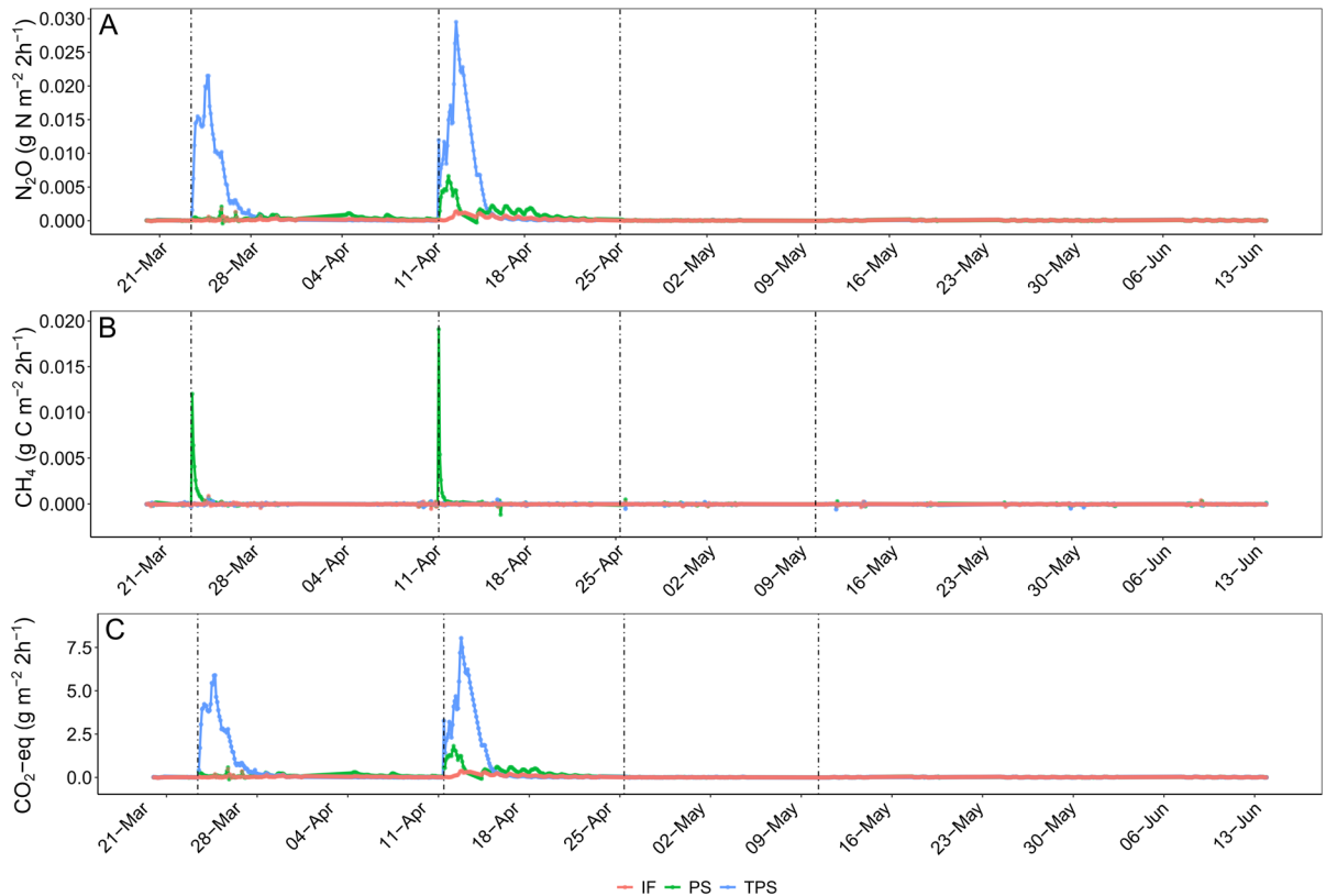
Fig. 1 2-h fluxes of A \text{N}_2\text{O} , B \text{CH}_4 and C \text{CO}_2 -equivalent fluxes of \text{N}_2\text{O} and \text{CH}_4 for each fertiliser treatment ( IF inorganic fertiliser, PS pig slurry, TPS treated pig slurry). Each data point represents the mean of three chambers used per
