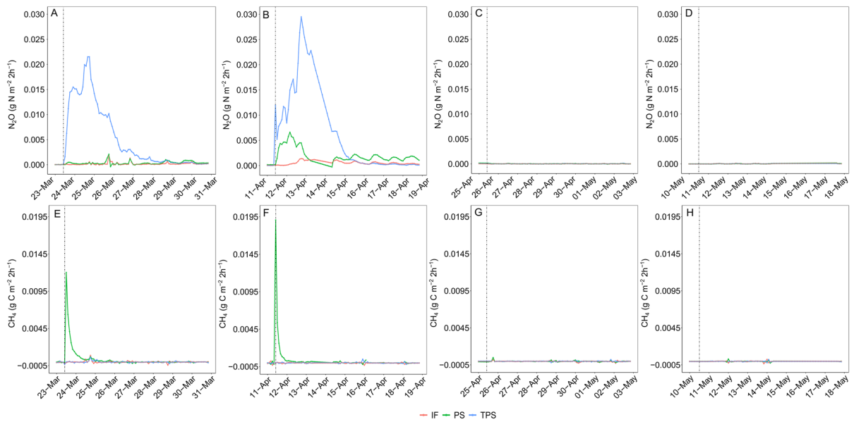
Fig. 2 2-h fluxes of A–D N_2O and E–H CH_4 during the first 7 days of each fertiliser application for each fertiliser treatment ( IF inorganic fertiliser, PS pig slurry, TPS treated pig slurry). Each data point represents the mean of three chambers
