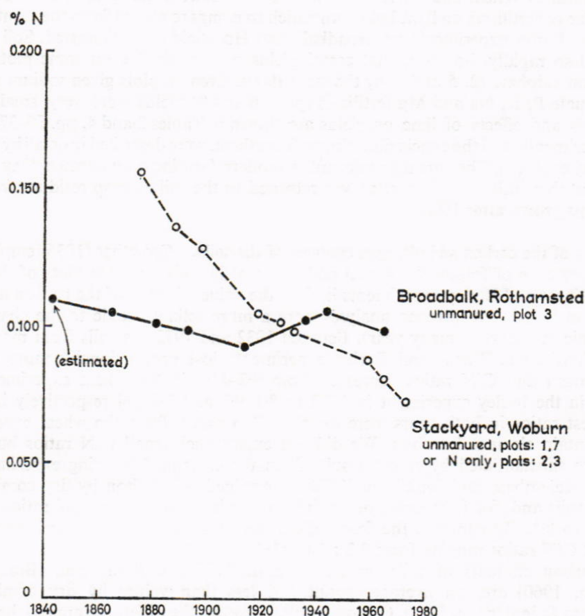
FIG. 2. Changes in nitrogen contents of soils from the Continuous Wheat and Barley experiments, Stackyard, Woburn, and from the Continuous Wheat experiment on Broadbalk, Rothamsted.
