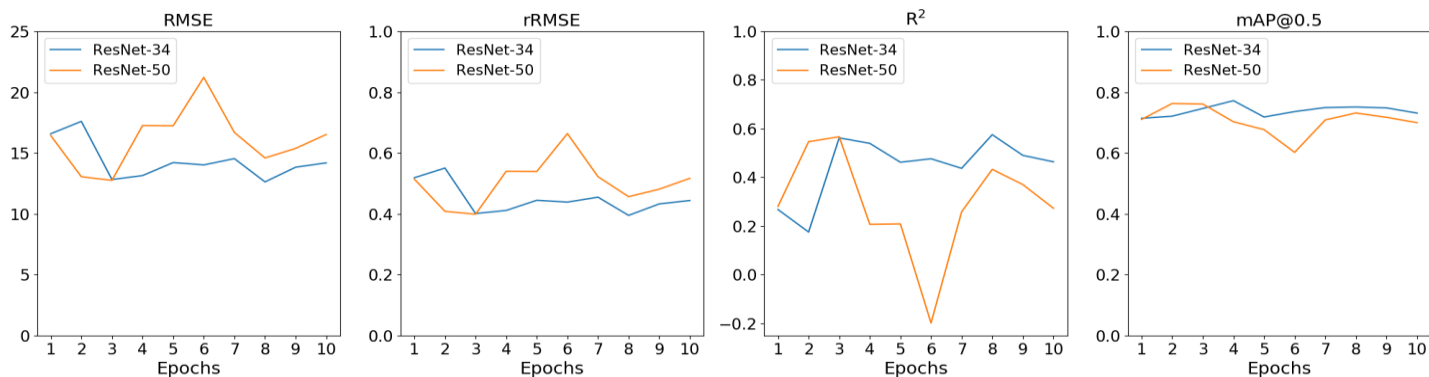
Figure S2: Epoch-wise results (RMSE, rRMSE, R^2 , mAP@0.5 ) of Faster-RCNN baseline with ResNet34 and ResNet50. The best model is obtained at epoch 3 for both backbones.
