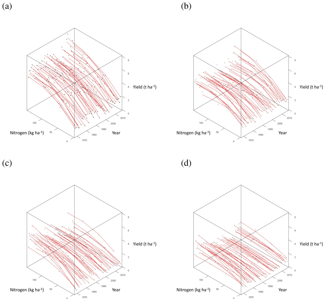
Fig. 8. Relationship between spring barley grain yield ( \bullet , t\ ha^{-1} at 85% dry matter) and applied nitrogen ( kg\ N\ ha^{-1} ) from Series O of the Hoosfield Long Term Experiment from 1968 to 2016 provided by the LEXP function (fitted curve, Eq. (3)) for each year separately from 1968 to 2016 for mineral fertilizer treatments (a) PKNaMg, (b) P, (c) KNaMg and (d) Nil. Model coefficients are given in Supplementary Table 3. Further details as Fig. 5.
