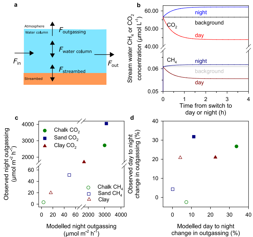
Figure 5. Simple reach-scale mass-balance modeling of diel changes in \text{CO}_2 and \text{CH}_4 . (a) Changes in water column \text{CO}_2 and \text{CH}_4 are products of benthic uptake or release ( F_{\text{streambed}} ); activity in the water column ( F_{\text{water column}} ), e.g., oxidation for \text{CH}_4 and net ecosystem metabolism (NEM) for \text{CO}_2 ; outgassing at the stream surface ( F_{\text{outgassing}} ); transport from upstream ( F_{\text{in}} ); and advective transport downstream ( F_{\text{out}} ). (b) Example of development of new steady-state concentrations for \text{CO}_2 and \text{CH}_4 after the switch from day to night for the Chalk River Wylye. Background is the initial ( t = 0 ) concentration in the water column ( C_{\text{background}} ), which is assumed equal to the concentration in water transported from upstream ( C_{\text{upstream}} ). (c) Modeled night outgassing rates versus observed mean outgassing rates during our high-resolution 2015 field campaign at the River Wylye (Chalk; green circles), Nadder (Greensand; blue squares) and Sem (clay; red triangles) for \text{CO}_2 (filled symbols) and \text{CH}_4 (open symbols). (d) The resultant change in rate of day to night outgassing, in percentage, for each gas based on (c).
