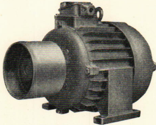
Fig. 4. Cowl-cooled squirrel cage induction motor.
