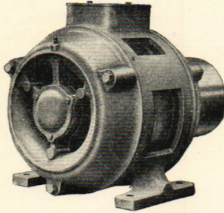
Fig. 2. Protected type squirrel cage induction motor.
