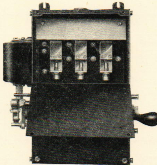
Fig. 6. Air break Star-Delta starter showing hinged lid.
