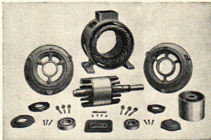
Fig. 1. Components of squirrel cage induction motor showing simple and robust construction.
