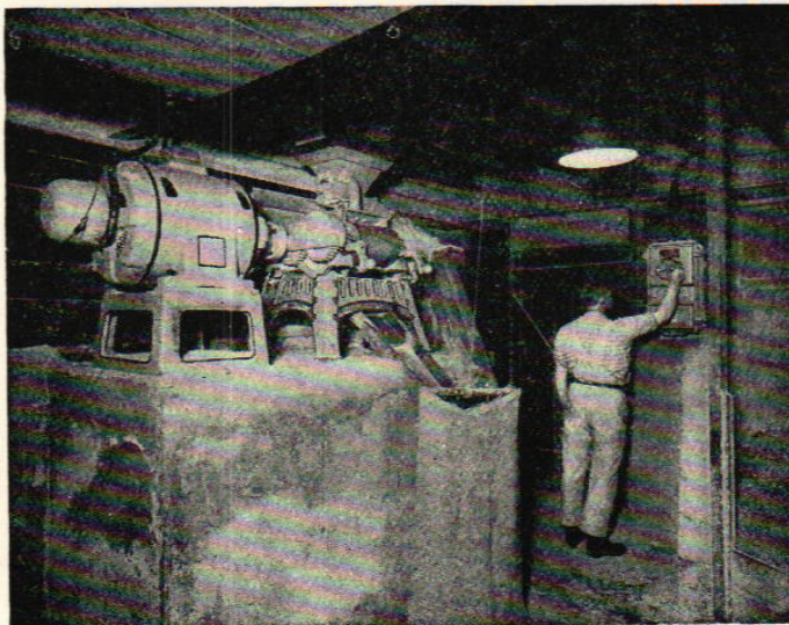
Fig. 13. 10 h.p. motor direct-coupled to grinder and crusher.
