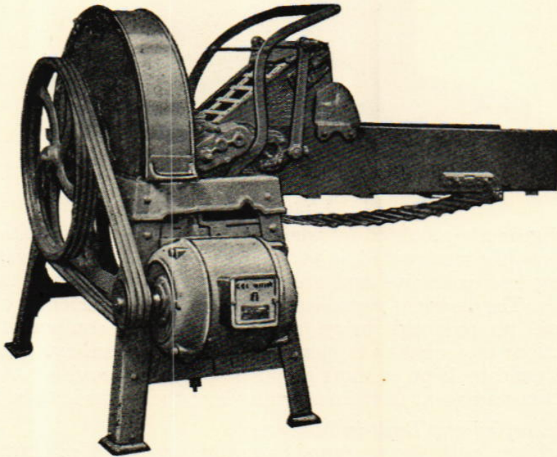
Fig. 14. Chaff cutter with vee rope motor drive.
