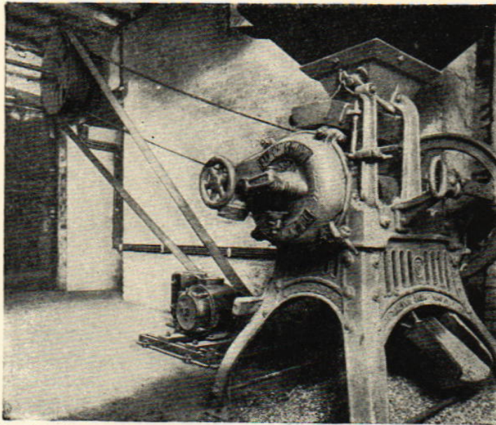
Fig. 8. Countershaft drive. Starter mounted on motor.
