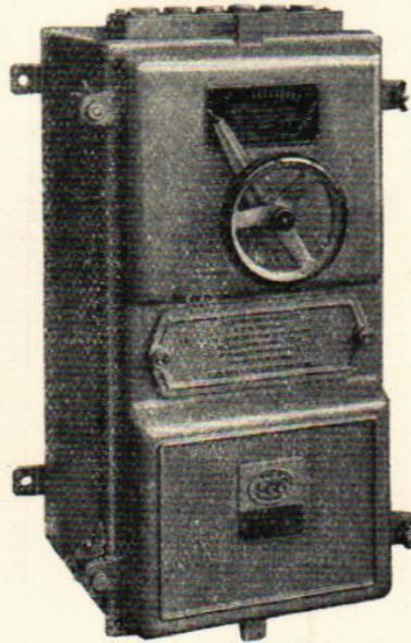
Fig. 7. Air break rotor and stator starting panel.
