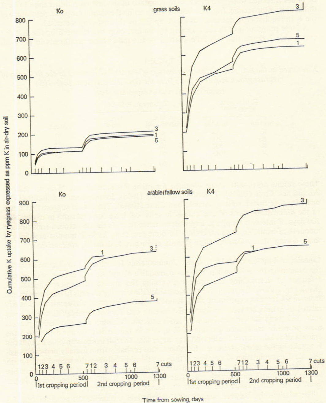
FIG. 1. Relationship between cumulative K uptake and time for soils without K ( K_0 ) or with 1043 kg K/ha ( K_4 ) applied in 1964 and cropped with grass or arable/fallow, 1958-67, from plots 1, 3 and 5 of the Classical Rotation experiment, 1848-1951, on Agdell.
