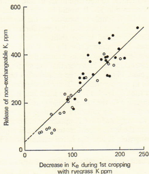
FIG. 4. Relationship between release of initially non-exchangeable K and the decrease in exchangeable K during the first cropping period by ryegrass ○ soils from arable/fallow sub-plots, ● soils from grass sub-plots.
